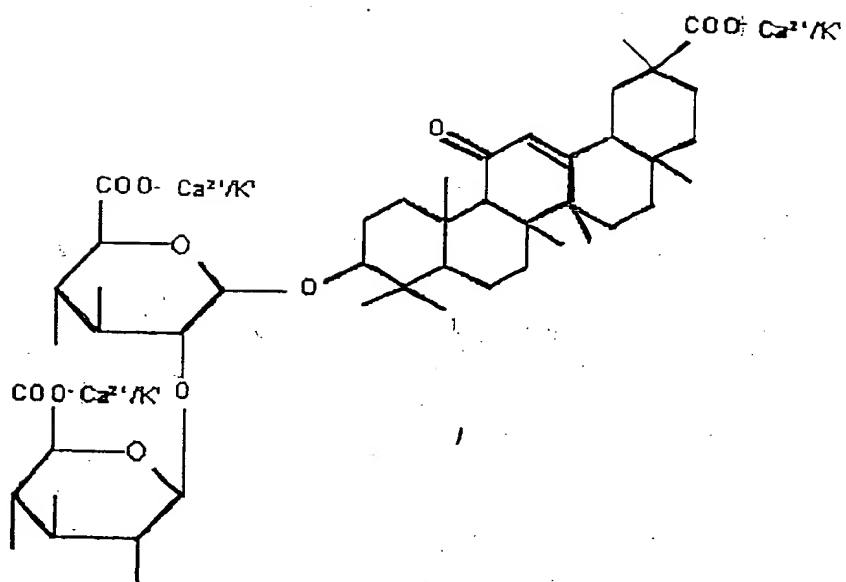
Glycyrrhizin = \text{Ca}^{2+} & \text{K}^+ salts of Glycyrrhizinic acid
